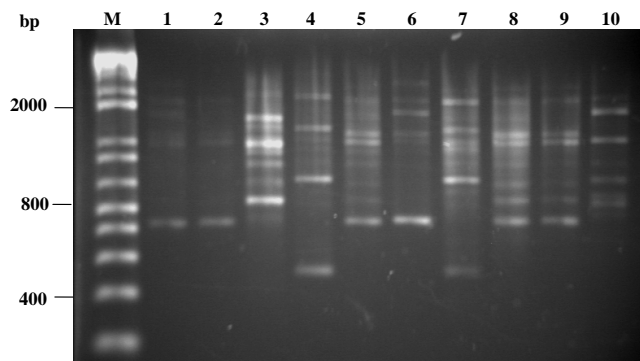
Figure 4. Products of RAPD-PCR amplification using the OPB07 and OPB09 primers. M, 100 bp molecular marker. The DNA template was (lane:isolate).- 1: MM0801, 2: AD0702, 3: AD0803, 4: CD0804, 5: FC0805, 6: FC0706, 7: AS0807, 8: GB0808, 9: L0909, 10: BC0710.
