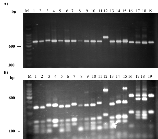
Figure 2. A) Products of amplification of the rDNA with the primers ITS1/ITS4 in different fungal isolates from Table 1. B) Amplified products of restriction (ARDRA) with the Hae II enzyme. M, 100 bp molecular marker. Lane: isolate.- 1: MM0801, 2: AD20802, 3: AD30803, 4: CD0804, 5: FC0805, 6: FC0706, 7: AS0807, 8: GB0808, 9: L0909, 10: BC0710, 11: SF0811, 12: YR0812, 13: ES0813, 14: AR0814, 15: JC0816, 16: M370, 17: M371, 18: M372, 19: M374.
