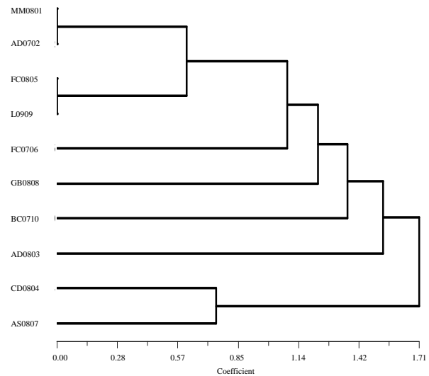
Figure 5. Dendrogram of fungal isolates obtained with the RAPD-PCR data using the Jaccard coefficient.
